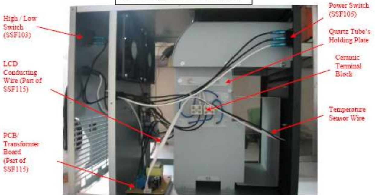
Inner Parts View – Side B
