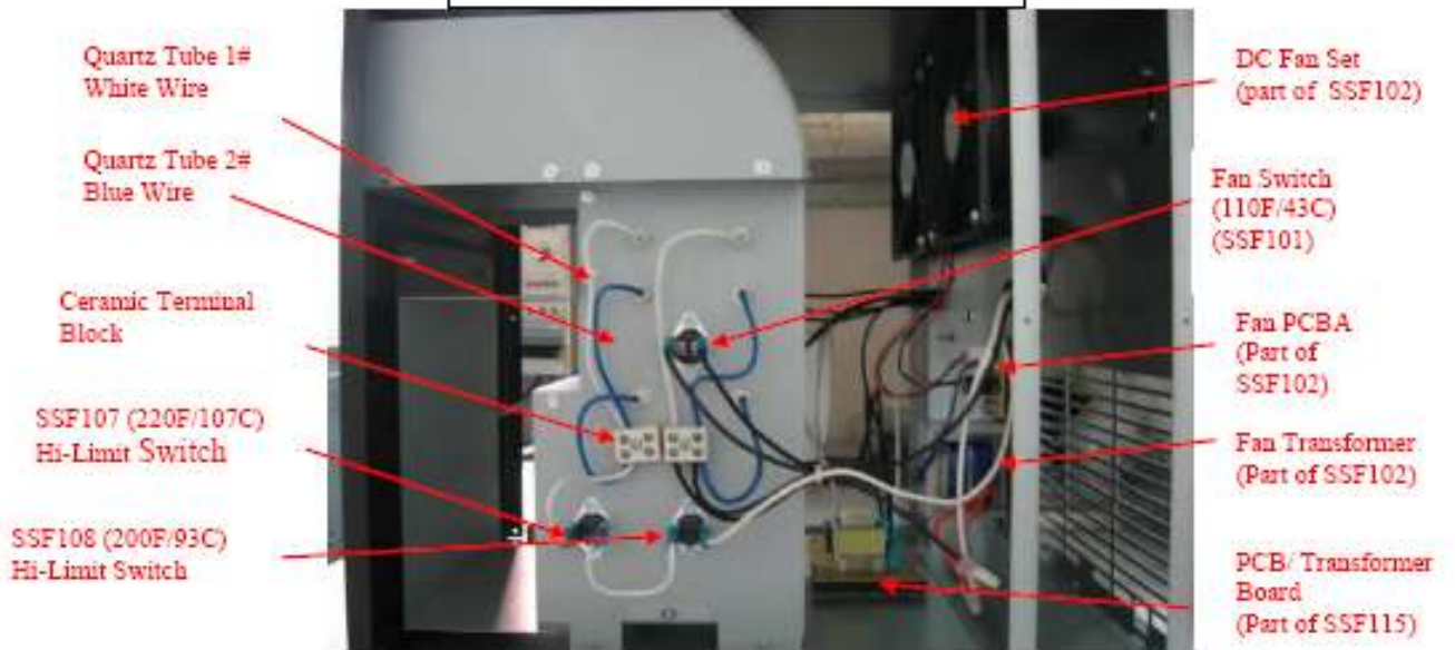
Inner Parts View – Side A
